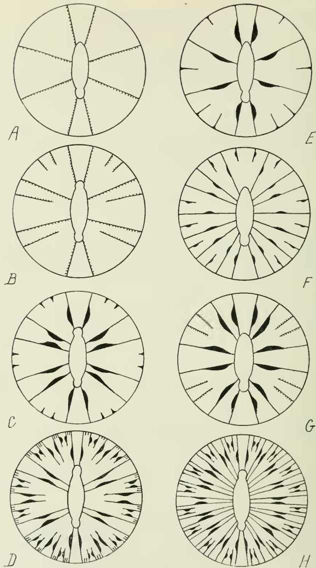
Diagrams of transverse sections showing various mesenterial formulae. A, supposed ancestor of Zoanthactinaria; B, Gonactinia ; C, Halcampa ; D, form with graded cycles of mesenteries but only six pairs perfect (e.g. Myonanthidae ); E, an Edwardsia ; F, Parazoanthus ; G, Carlgrenia ; H, form with graded cycles of mesenteries, and sixteen pairs perfect. Compare this with a further stage shown in Text-fig. 10.
